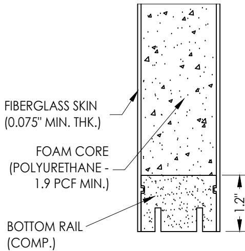
2 3 VERTICAL CROSS SECTION
