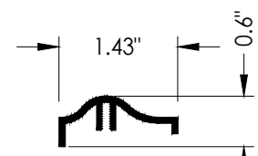
2B DECORATIVE TRIM PVC
