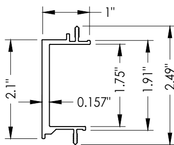
2A MOUNTING CHANNEL ALUM (6063-T6)
