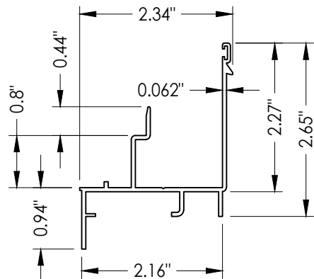
2C FRAME SILL ALUM (6063-T6)
