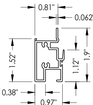
2F MEETING RAIL ALUM (6063-T6)
