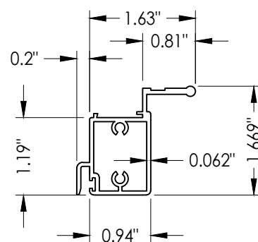
2D VENT BOTTOM RAIL ALUM (6063-T6)
