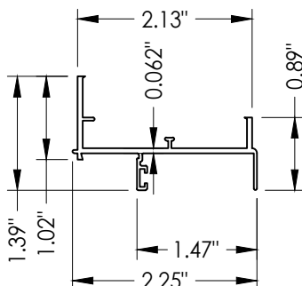
2G FRAME HEAD ALUM (6063-T6)
